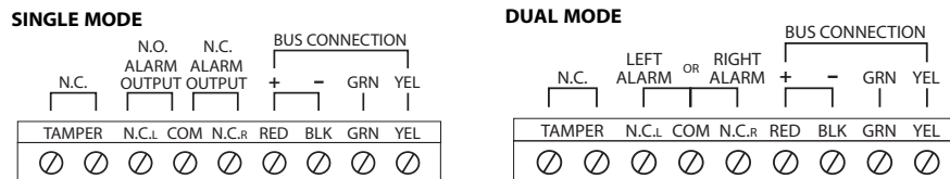
Figure 1: Wiring Methods
