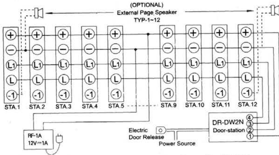
Figure-5 TP-nRC and DR-DW2N Connection Diagram
